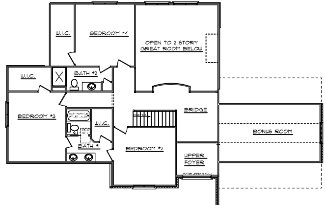
2ND FLOOR PLAN (ALTERNATE LAYOUT - 13706F)
