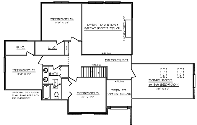
2ND FLOOR PLAN (12306F)
