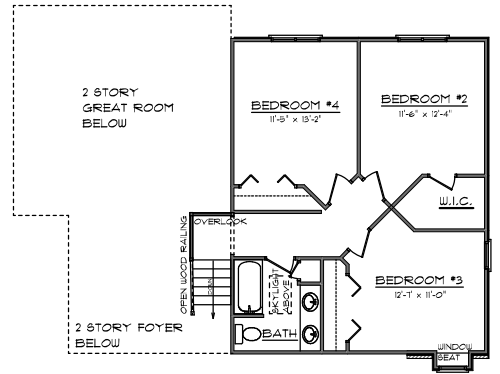
2ND FLOOR PLAN OPTION #1 (3 BEDROOMS)
