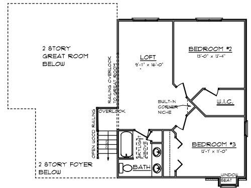
2ND FLOOR PLAN OPTION #2 (2 BEDROOMS W/LOFT)
